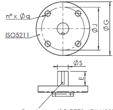
Parallel key ISO R773 / DIN6885A
